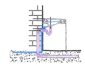
TUBERIA PVC SAL S=2%
